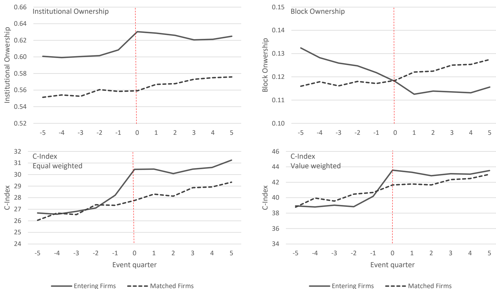
Fig. 7: Firm-level Cross-ownership Index and institutional ownership around S&P 500 additions.
